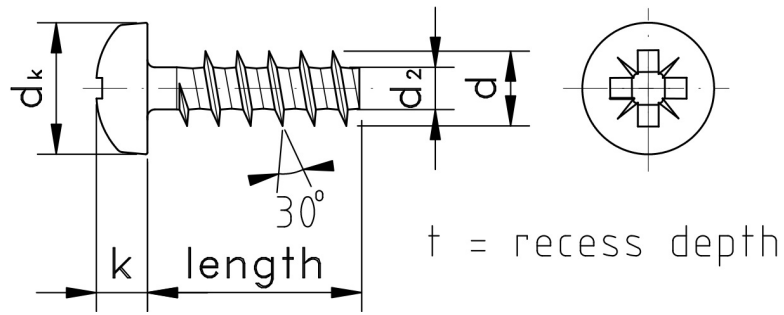
Figure 1: Pozi Pan Thread Forming Screw for Plastics
