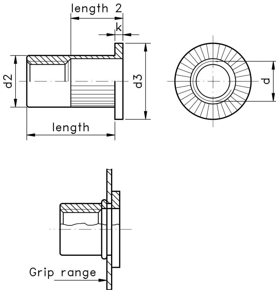
Figure 1: Rivet nuts with flat head, knurled shank and an open end
